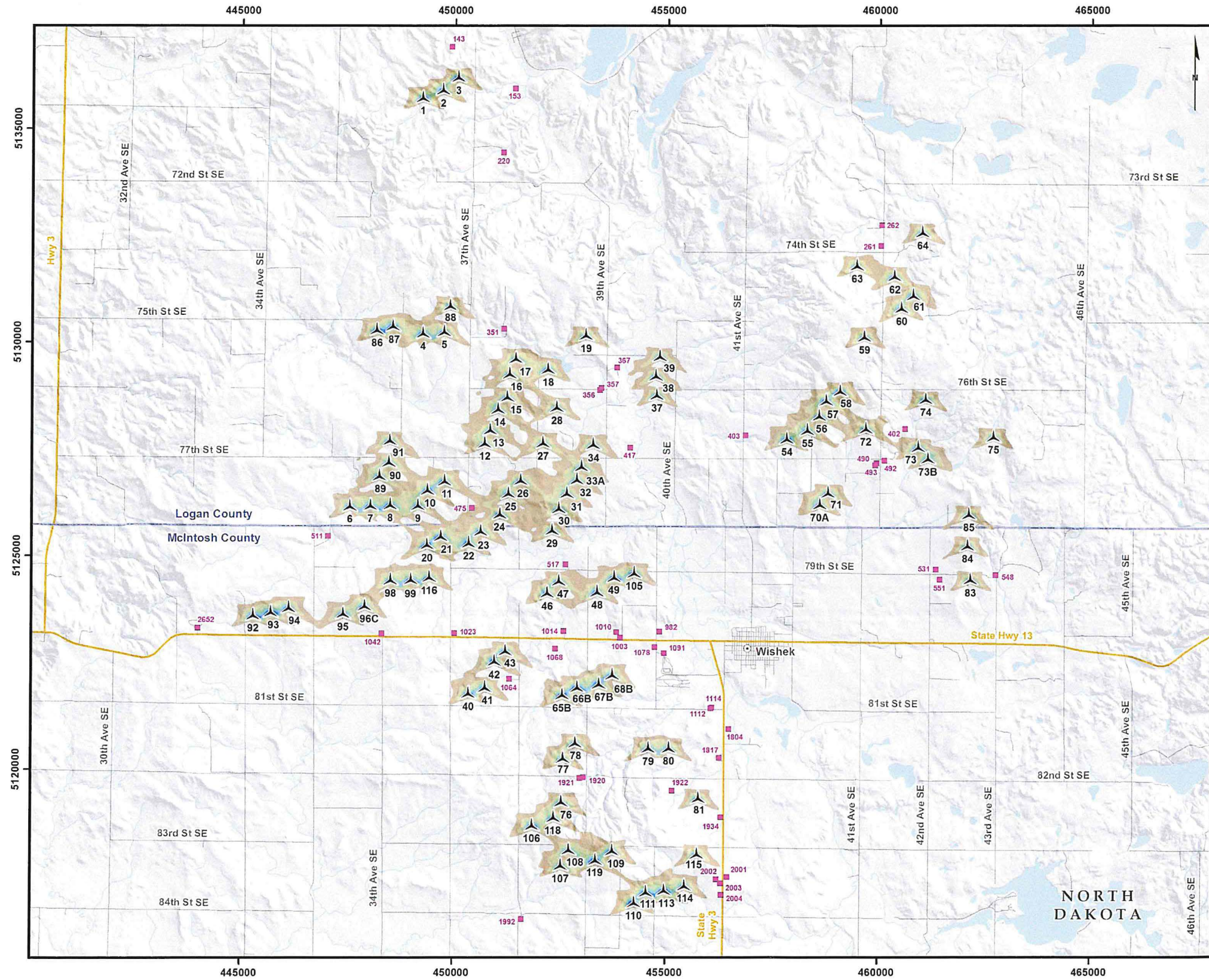
Figure 4-1 Modeled hours of shadow flicker (Expected Case)
